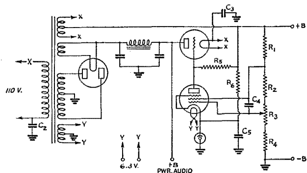
FIG. 1.—REGULATED PLATE SUPPLY WITH CHANGES SUGGESTED BY W9KNZ
